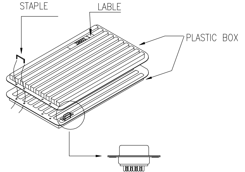
DETAIL B
